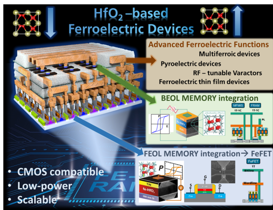
Illustration of HfO 2 -based ferroelectric devices enabling scalable, CMOS-compatible non-volatile memory. The architecture supports integration in both front-end (FeFET) and back-end memory structures, while opening pathways to advanced ferroelectric functionalities such as multiferroic, pyroelectric, and tunable RF devices. © Fraunhofer IPMS
