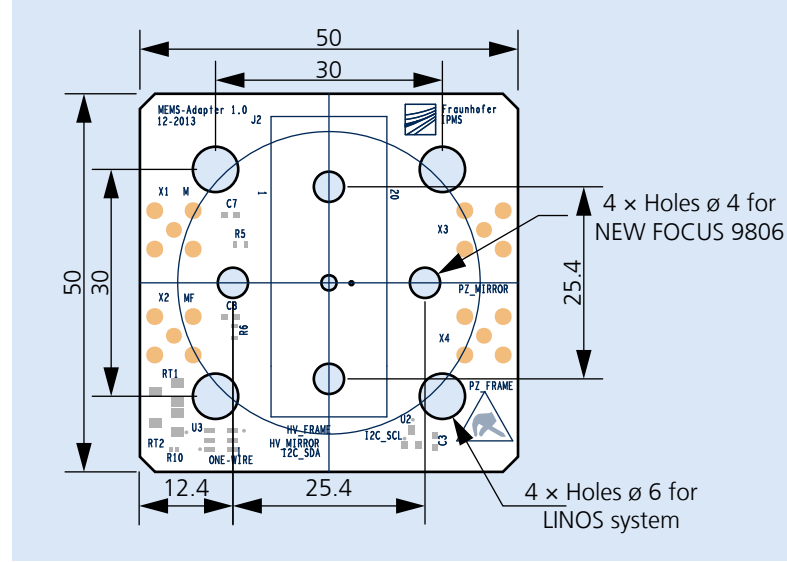
Schematic drawing of MEMS adapter board
