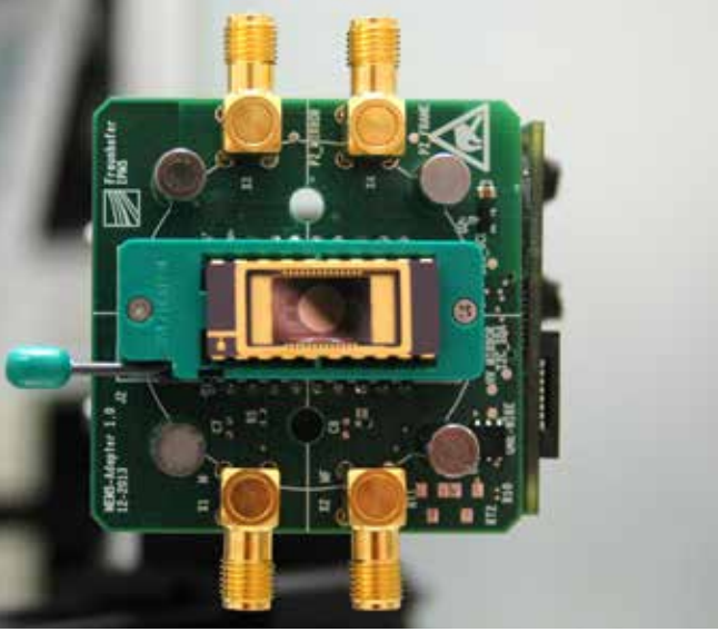
View of MEMS adapter board
