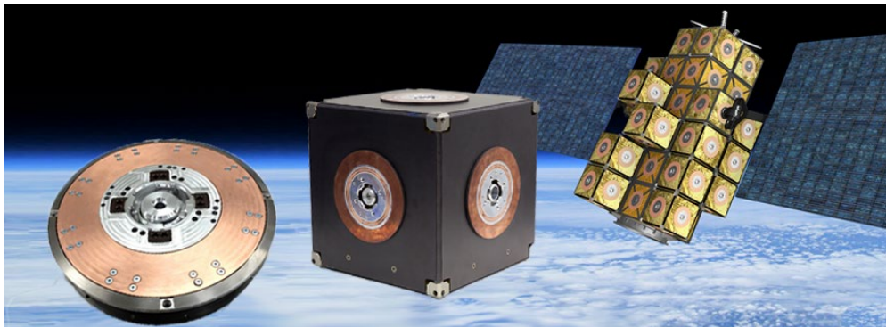
iSSI® (intelligent Space System Interface) from iBoss GmbH, in which the LiFi Gigadock® transceiver from Fraunhofer IPMS is integrated. © iBoss GmbH
